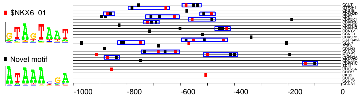
Figure 5: Visualization of the two motif CRM that we learned for the regulation of CDK activity annotation. Shown are the 1000bp upstream regions of all 28 genes that are assigned to this annotation according to GO. The occurrences of the two motifs in each upstream region is shown as red (NKX motif) and black (novel motif) rectangles, where we highlighted (blue rectangle) all 13 genes in which the two motifs occurred within 200bp of each other in the gene’s upstream region.
