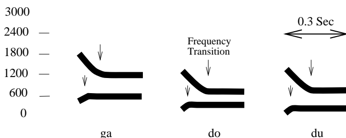
Figure 1.2: Synthetic spectrograms using only F1 and F2 information that produced the voiced stops before various vowels (from [30]).
