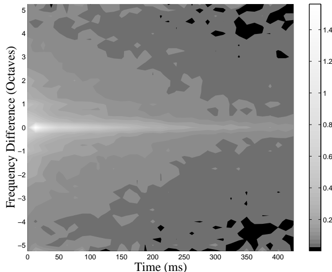
Figure 1.3: The time-frequency information density of a randomly selected 2-hour section of the Switchboard corpus, in bits per unit area (from [5]).
