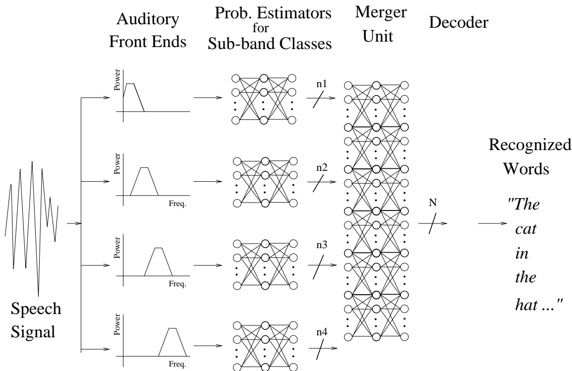
Figure 3.3: Merging on the frame level using an MLP.
