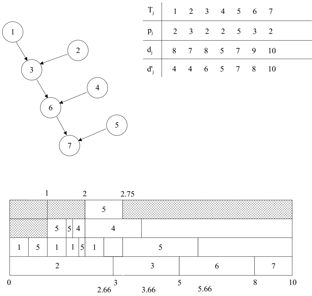
Figure 4: Minimizing L_{max} on an increasing zigzag pattern
