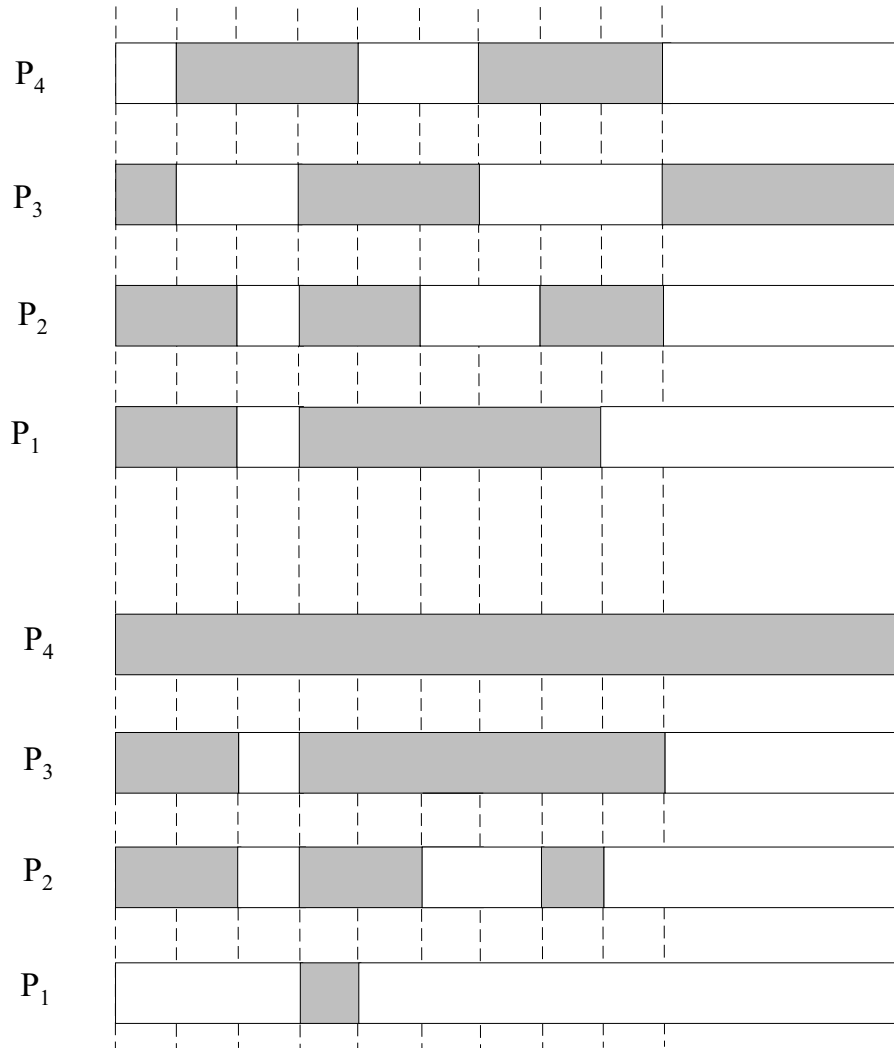
Figure 1: Rearrangement of arbitrary patterns
