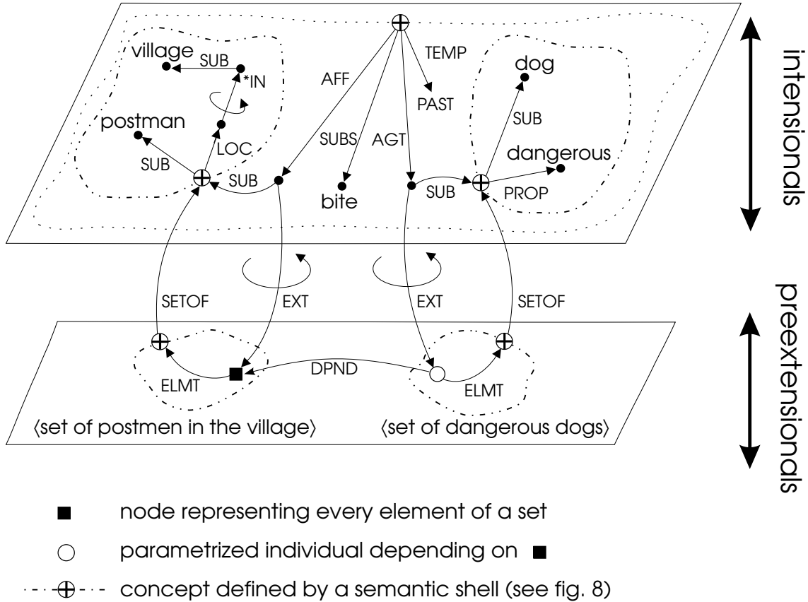
Figure 7: Using Parametrized Nodes for the Representation of Mixed Quantification
