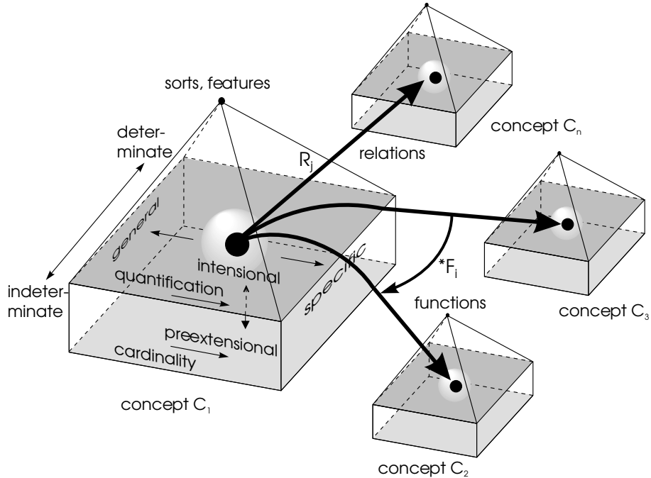
Figure 2: Basic Representational Means of MESNET
