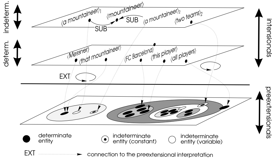
Figure 5: Referentiality and Types of Nodes in the Preextensional Layer
