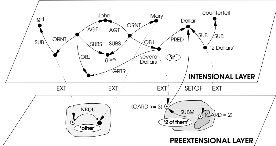
Figure 4: Intensional and Preextensional Representatives
