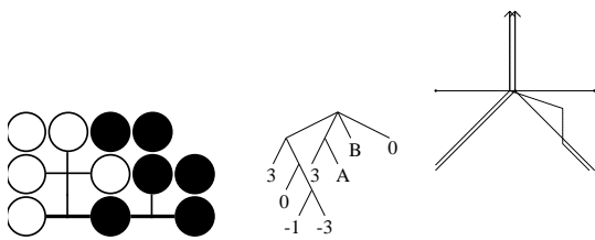
Figure 82: Unnamed ko. Remark: A and B are positions in the game graph of the "2-iterated ko".
