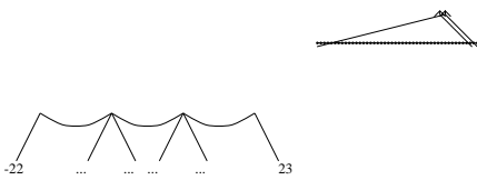
Figure 56: Hot 3-iterated ko, node 1.2
