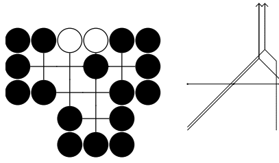
Figure 78: Takizawa's Rogue, node 1.1
