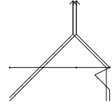
Figure 88: Real 9, node 1 (B is position in 2-iterated ko)
