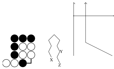
Figure 106: 3 Points Without Capturing, node 1
