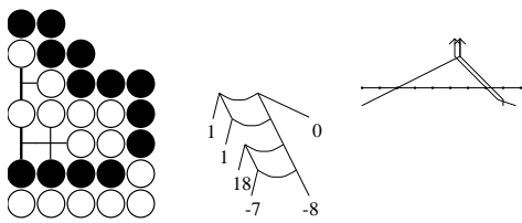
Figure 66: Approach ko, node 1.1
