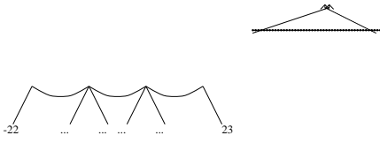
Figure 55: Hot 3-iterated ko, node 1
