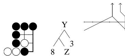
Figure 108: 3 Points Without Capturing, node 1.2.1.1
