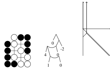
Figure 81: Kato - Fujisawa, node 1.3
