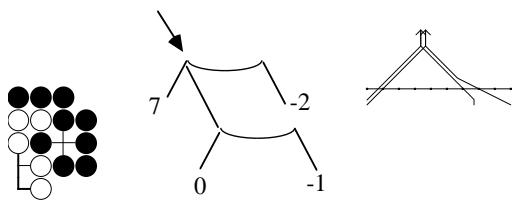
Figure 43: Kim Yonghoan's ko, node 1.1
