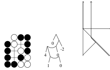
Figure 80: Kato - Fujisawa, node 1
