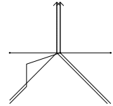
Figure 89: Real 9, node 1.2 (B is position in 2-iterated ko)
