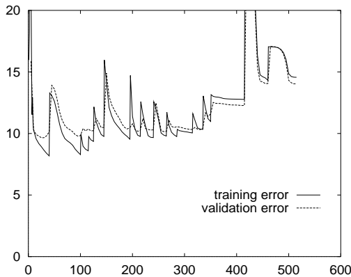
Figure 2: Development of training and validation set error over time for the same run of autopruning from which the figures above were derived. x -axis: number of epoch, y -axis: Error. There are 15 pruning steps after which 15% of the initial connections remain. In this example pruning is not successful: no lower validation set error occurs than before the first pruning step. This is not a rare case.
