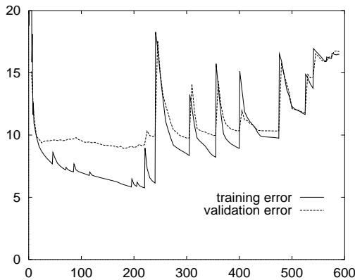
Figure 3: The corresponding curves for lprune . There are 21 pruning steps, initially removing only few connections, later removing more in each step. Finally, 0.5% of the initial connections remain. Pruning is successful: after 7 pruning steps (in epoch 180) a lower validation set error is reached than before the first pruning step.
