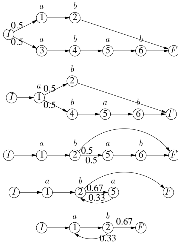
Figure 1: Model merging for HMMs.
