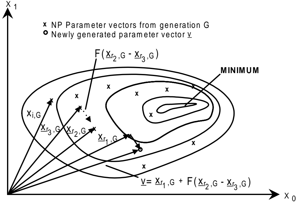
Fig.1: Two-dimensional example of an objective function showing its contour lines and the process for generating \underline{v} in scheme DE1. The weighted difference vector of two arbitrarily chosen vectors is added to a third vector to yield the vector \underline{v} .
