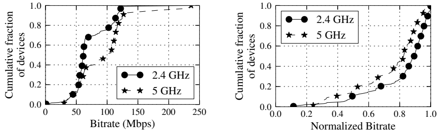
Fig. 6: Distribution of wireless bitrates for devices in both the 2.4 GHz and 5 GHz spectrums, for all devices in the deployment. Devices in the 2.4 GHz spectrum see lower bitrates.
