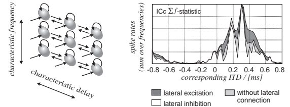
Figure 3: Left: Formation of a 2-dimensional map representing the tonotopy and characteristic delays. Right: The lateral interconnections cause a sharpening or smoothing of the ITD-feature. The response to high frequencies contains periodical components – since the coincidence detection is similar to a cross-correlation of periodical signals, its result is just as periodical.
