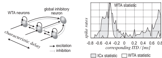
Figure 5: Left: Structure of the WTA network. Right: Result of the selection process.
