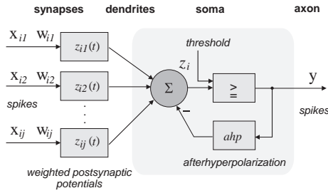
Figure 2: Neuron model
