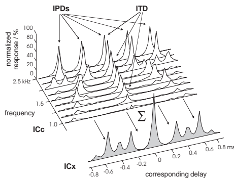
Figure 4: The combination of the tonotopic distributed response of the ICc in a one-dimensional ICx-model enables to distinguish ITD from phase differences (IPDs).
