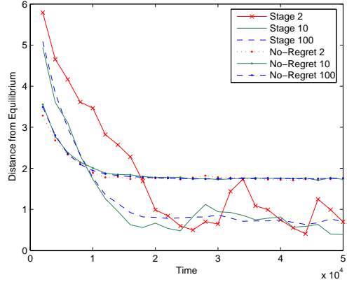
Figure 2: Convergence with random matching
